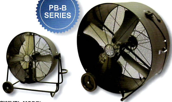
STANDARD MODEL
